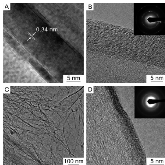
Figure 7. (A) HRTEM image of graphite showing its characteristic 0.34-nm interlayer spacing. (B) HRTEM image illustrates the intercalation of GO samples oxidized for more than 96 h. The GO sheets are wrinkled compared to that of pristine graphite. The SAED pattern in the inset contains information from many GO grains. (C) TEM image of FGS. (D) An edge-on HRTEM image of FGS produced from GO with a 96-h acid treatment showing a multi-stack region.
